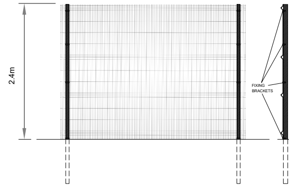
Weld Mesh Security Fencing
