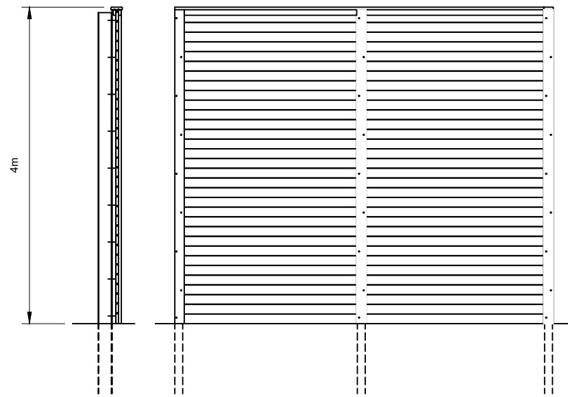
Acoustic Fencing Indicative Design
