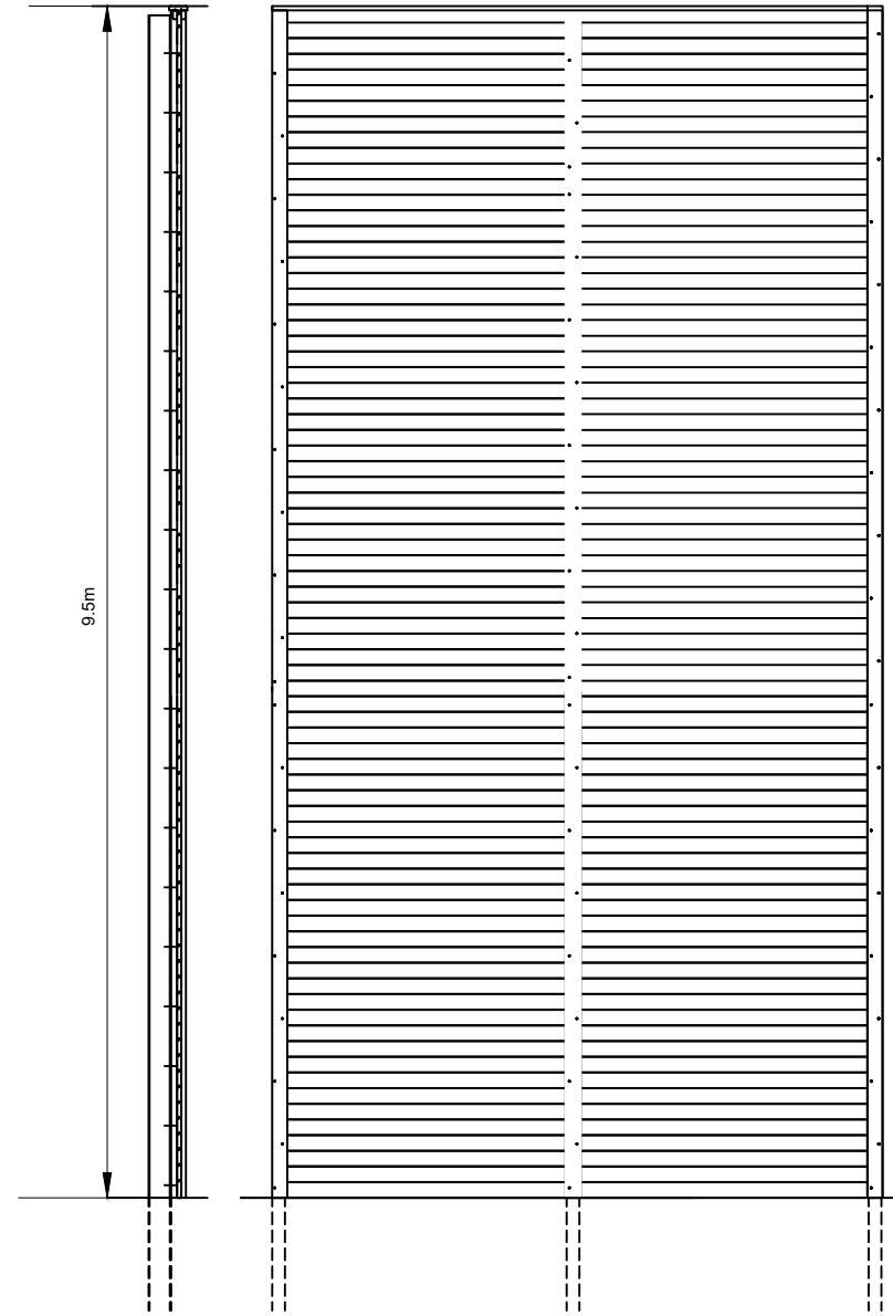
Blast Wall Indicative Design
